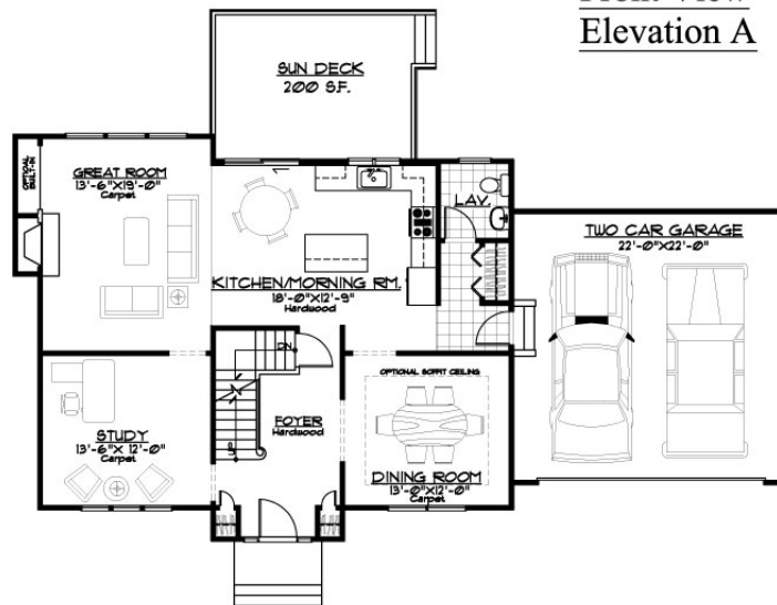
First Floor 1,110 S.F.
