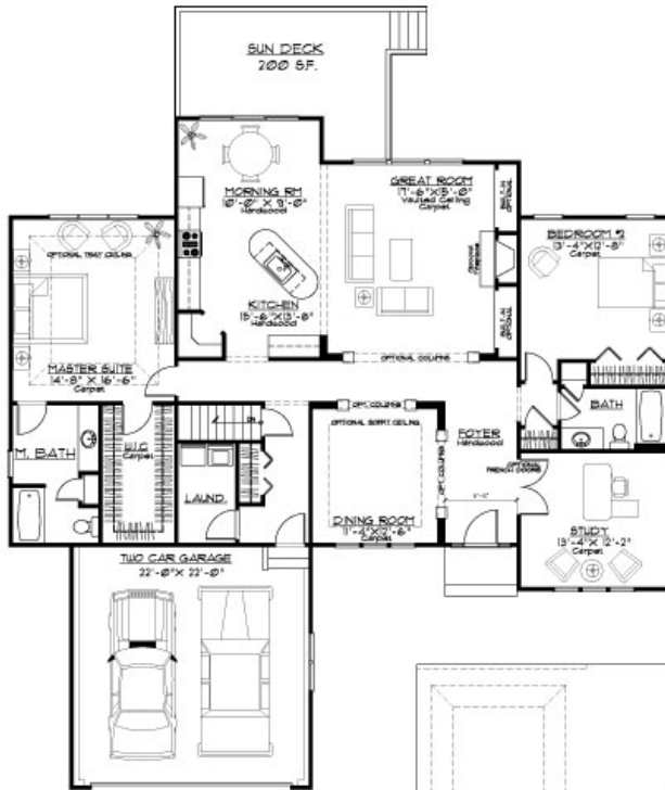
First Floor 2,100 S.F.
