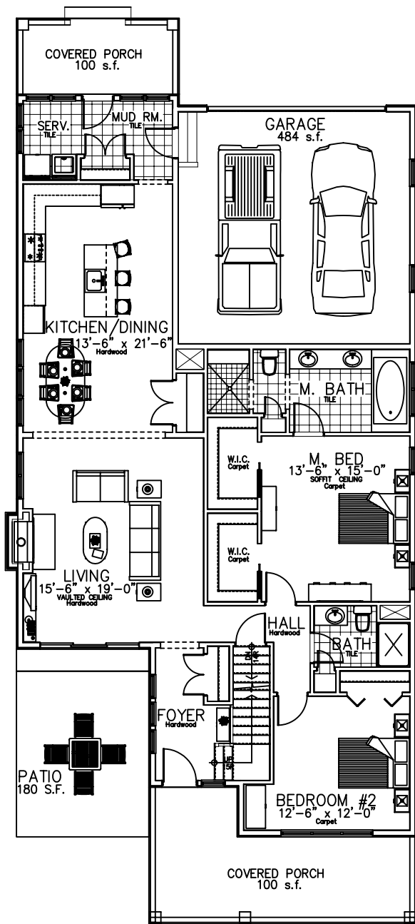
FIRST FLOOR 1,680 s.f.
