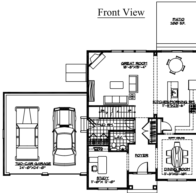
First Floor 1,214 S.F.
